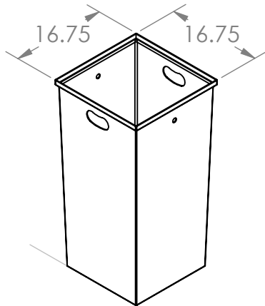
OPTIONAL LINER: 16 X 16 X 34" HIGH
